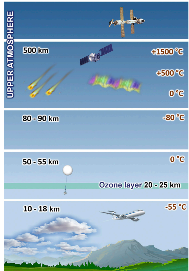
Figure 54 Atmospheric Layers
