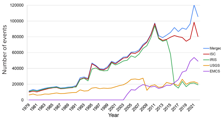
Comparison of the number of M3+ earthquakes from 1979 to 2022 based on data from various seismic databases
