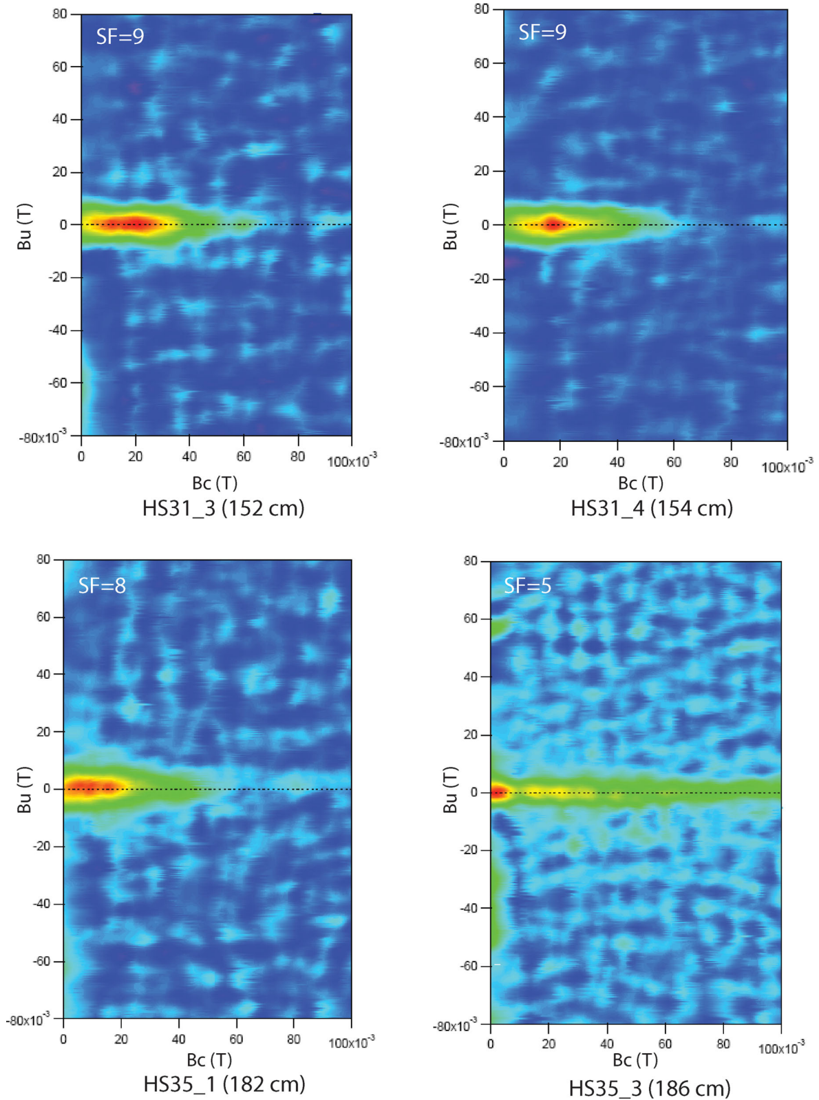
Figure 6. First order reversal curve (FORC) diagrams for same representative specimens discussed in Fig. 5. The FORC data have been processed using the FORCinel software (Harrison & Feinberg 2008). SF, smoothing factor. Lacustrine sediments samples are characterized by a coercivity distribution with almost closed contours peaked at coercivity B_c of about 15–25 mT. The FORC diagram for the sample HS35_3, just on top of tephra SUL2–20, shows a restricted peak close to the origin and a long tail along the B_c axis, extending beyond 100 mT.
